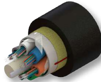
Cables ADSS
