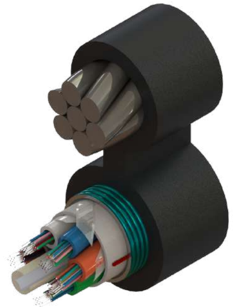
CABLE FIGURA 8 ARMADO 1/4" 72F G652D S EX
