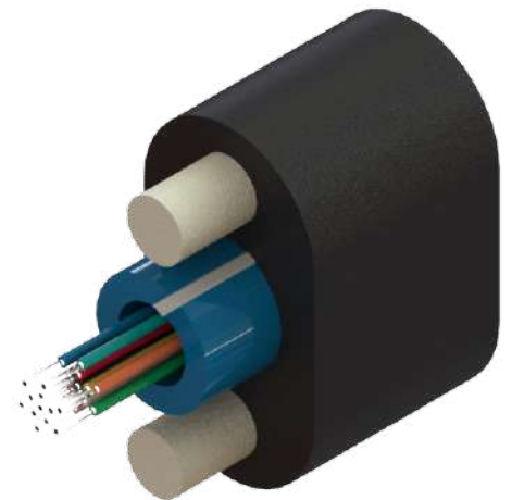
CABLE FLAT DROP 3.0MM 12F G652D D00002 S EX
